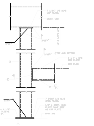
9 DETAIL - COLUMN C1 DIMS: 1'-0" x 1'-0"
