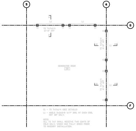
8 PLAN - GENERATOR ROOM LOUVERS DIMS: 4'-0" x 4'-0"
