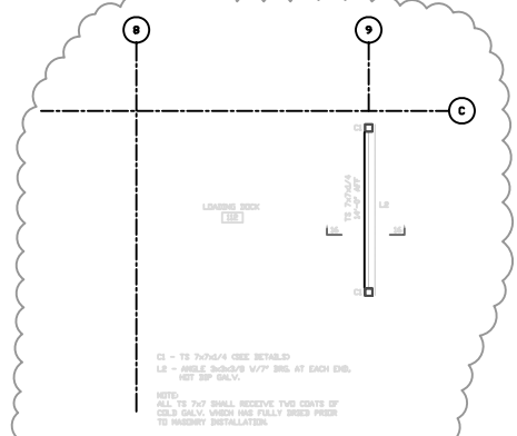
13 PLAN - LOADING DOCK OVERHEAD DOOR DIMS: 4'-0" x 4'-0"
