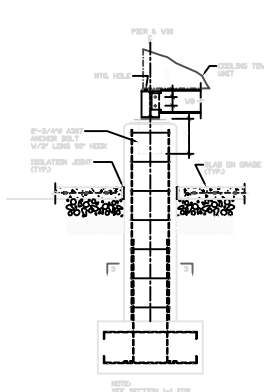
6 SECTION 2-2 DIMS: 4'-0" x 1'-0"
