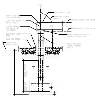
5 SECTION 1-1 DIMS: 4'-0" x 1'-0"
